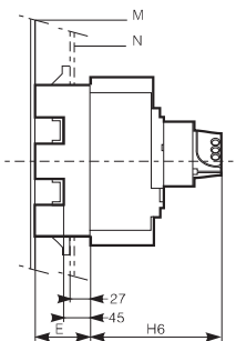
CFM5-100~630 3P Vigi CFM5-100~630 3P
