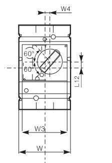
CFM5-100~630 3P Vigi CFM5-100~630 3P
