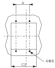
• CFM5E-100~630 4P
