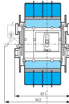
• CFM5E-100~630 4P
